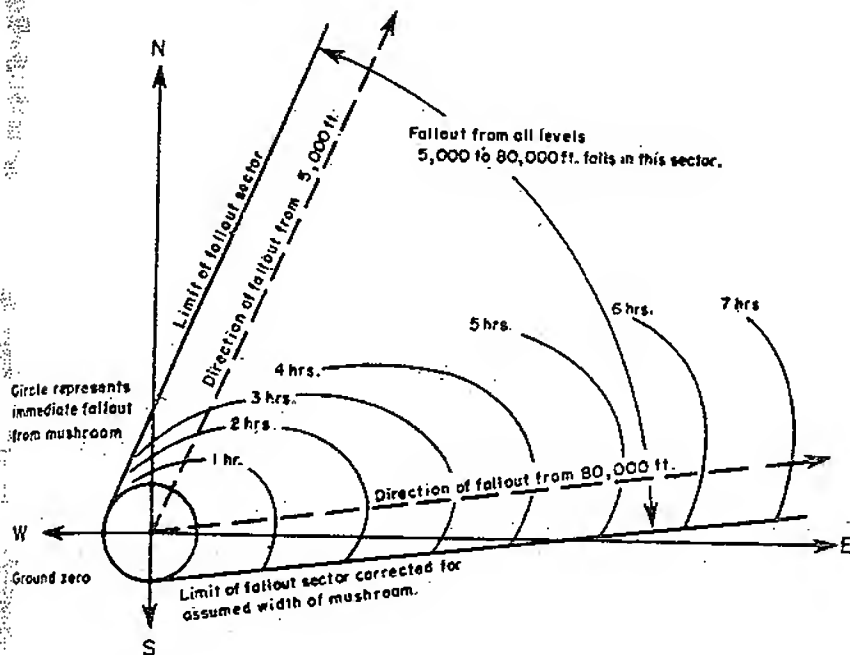
Figure 5. Sector of fallout from stem of cloud.
